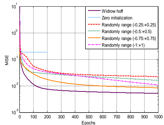
Fig. (6) Effect of Initialization Weight Functions
