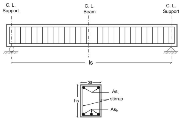
Fig. (5) Dimensions of Spandrel Beam
